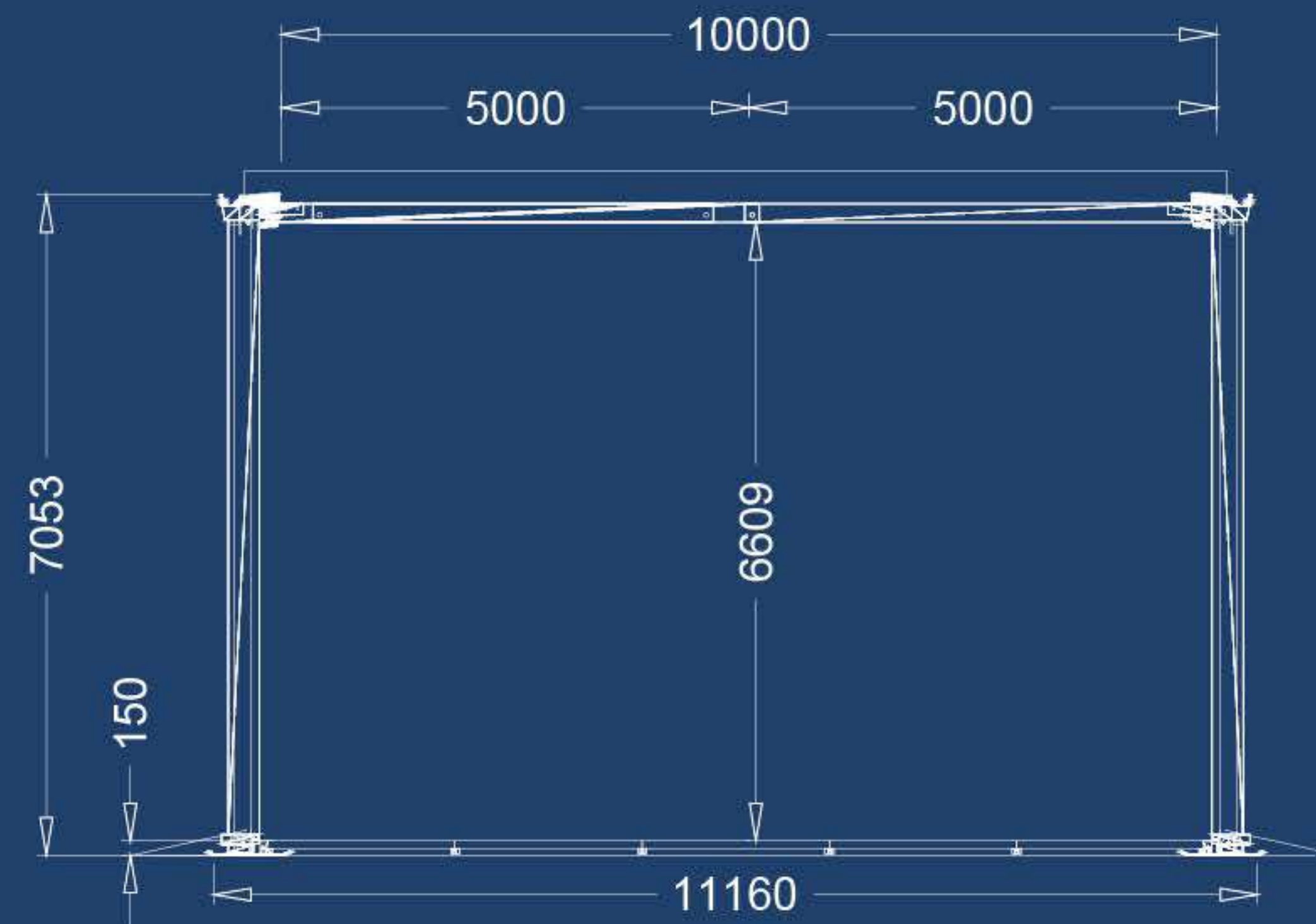
10m porch without mezzanina
