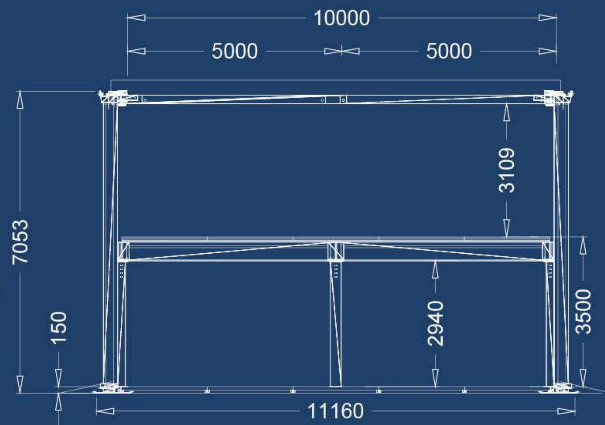
10m porch with mezzanina
